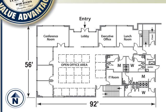
OFFICE PLAN 5,235 SF
