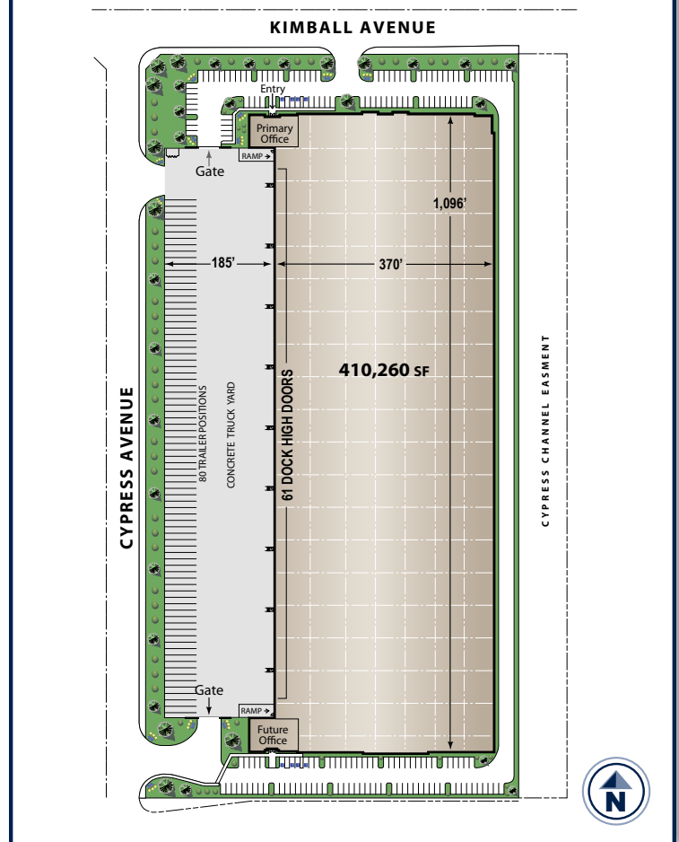
LEGACY BUILDING SM 827 SITE PLAN
