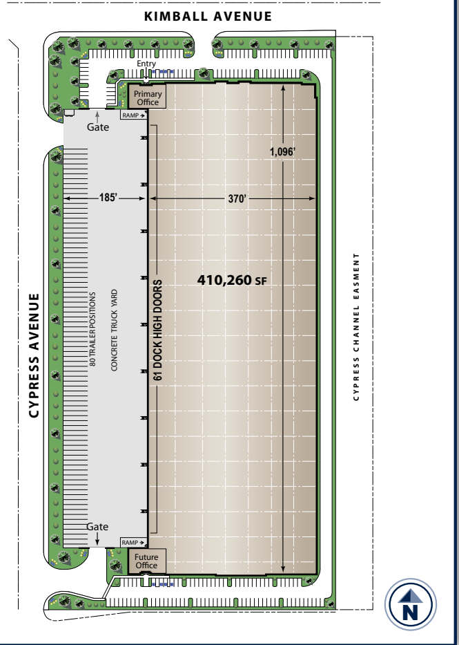
LEGACY BUILDING SM 827 SITE PLAN
